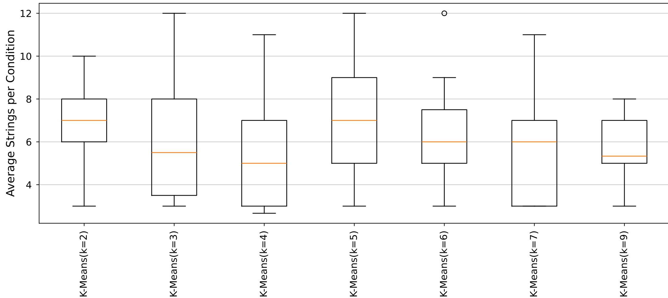
YARA Rules Average Strings per Condition Distribution (Cluster14_Size9 dataset)
